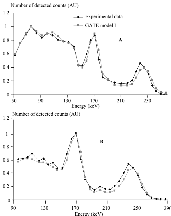
Fig. 3. Acquired and simulated spectra of LINE1w (A) and CYL (B) when using GATE model I.
